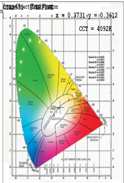
CIE1931 Chromaticity Diagram
